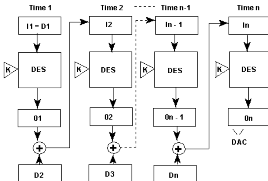
APPENDIX 1 BLOCK DIAGRAM OF THE DAA
