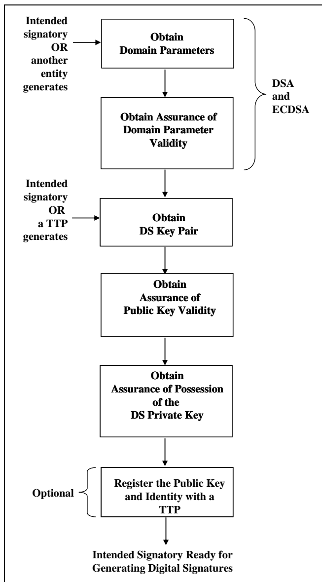
Figure 2: Initial Setup by an Intended Signatory
