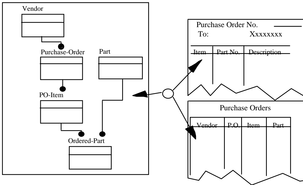
Figure A3.10. Scope of a Function View
